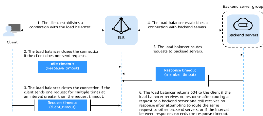
Figure 1-7 Timeout durations at Layer 7
